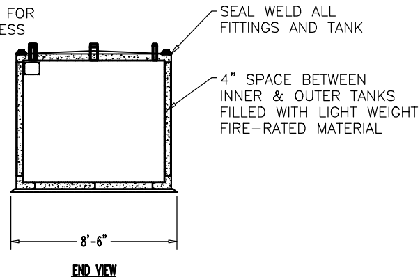
END VIEW
