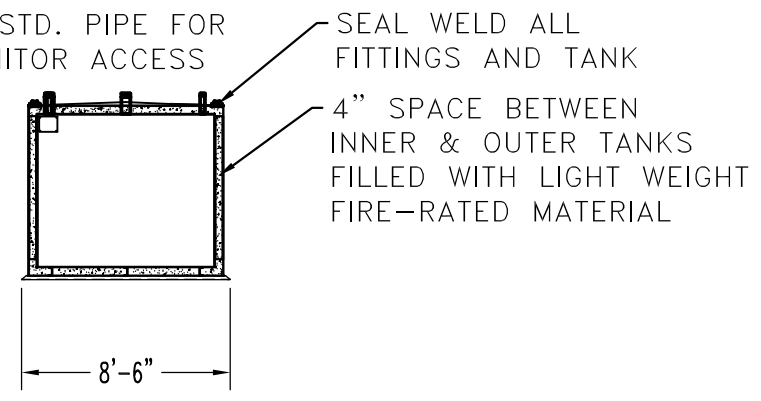
END VIEW
