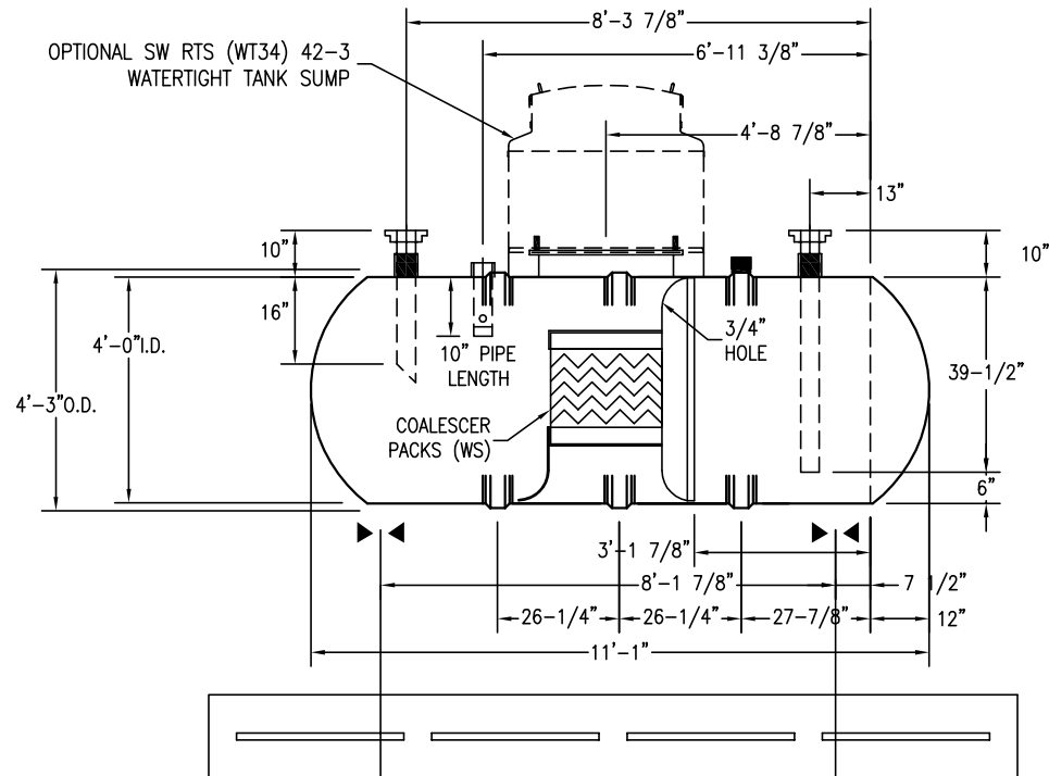
OPTIONAL 18"x 8"x 14' DEADMAN
