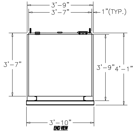
END VIEW
