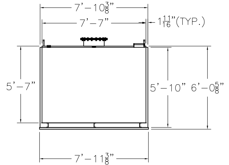
END VIEW
