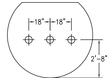
"BAFFLE DETAIL"
