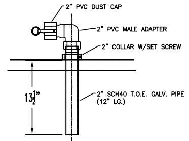
DETAIL A SCALE 1:12
