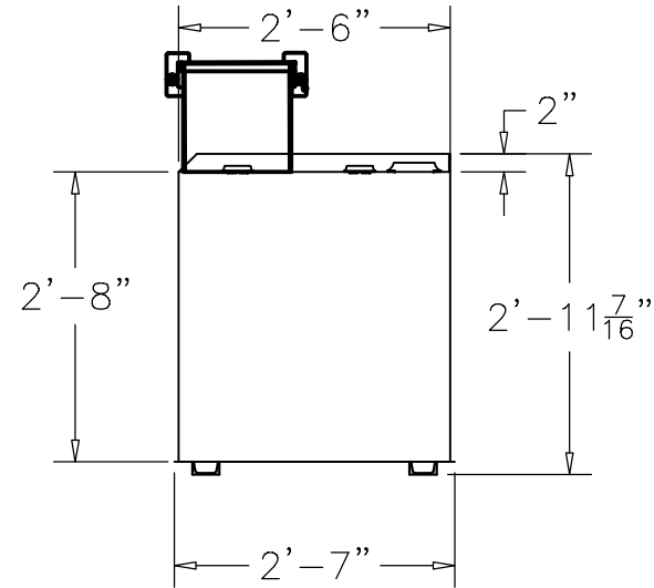
END VIEW
