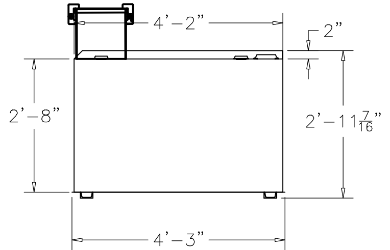
END VIEW
