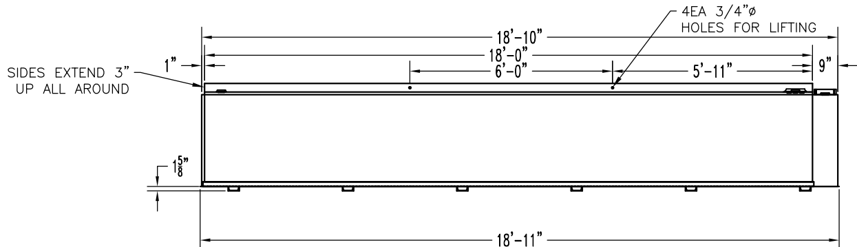
ELEVATION VIEW
