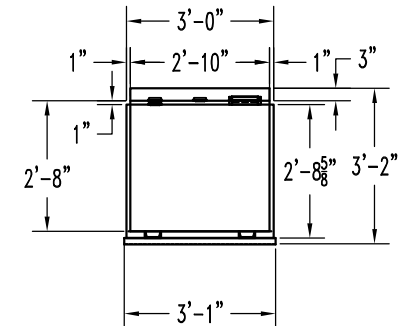
END VIEW
