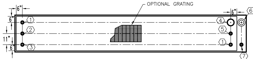
TOP VIEW
