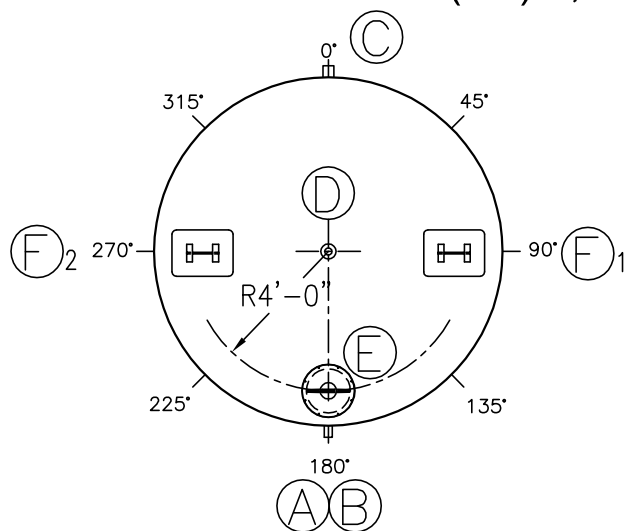
TOP VIEW (TRUE ORIENTATION)
