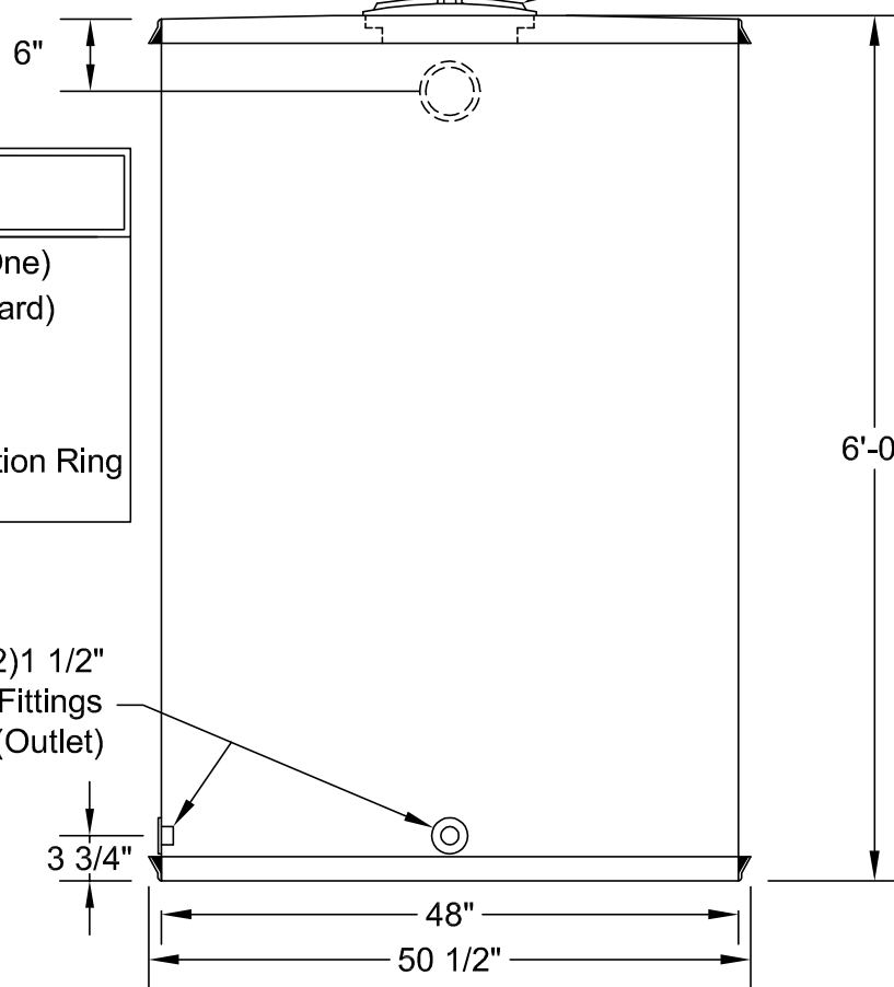
ELEVATION VIEW
