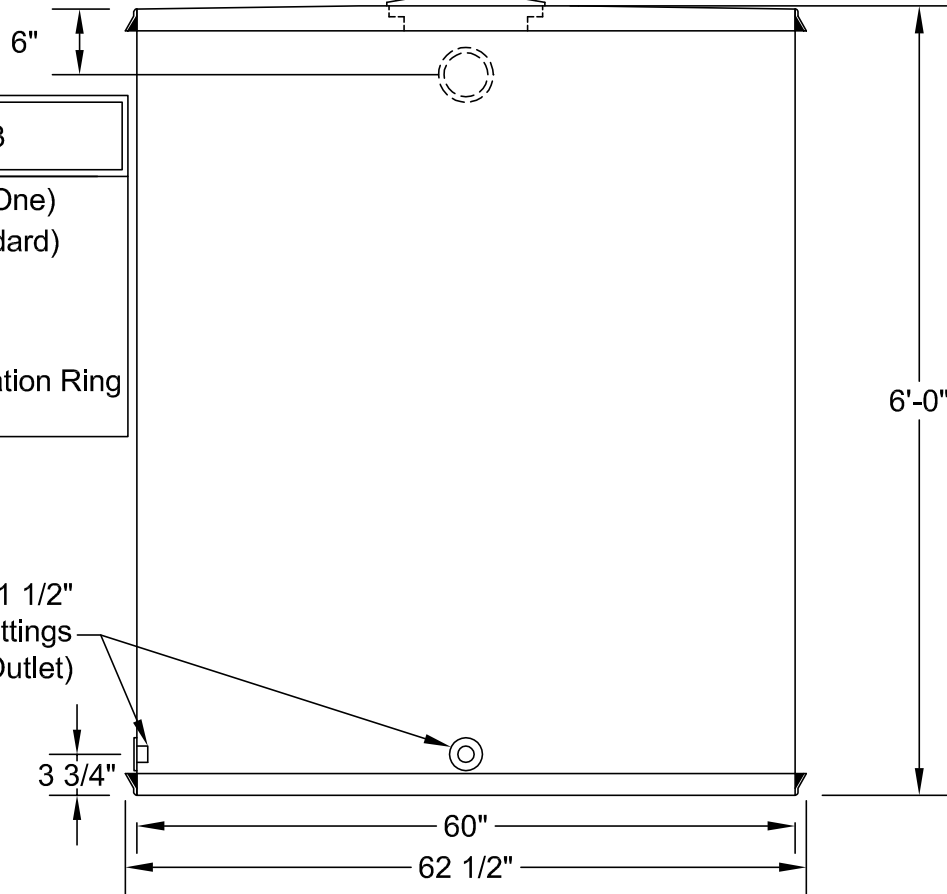
ELEVATION VIEW
