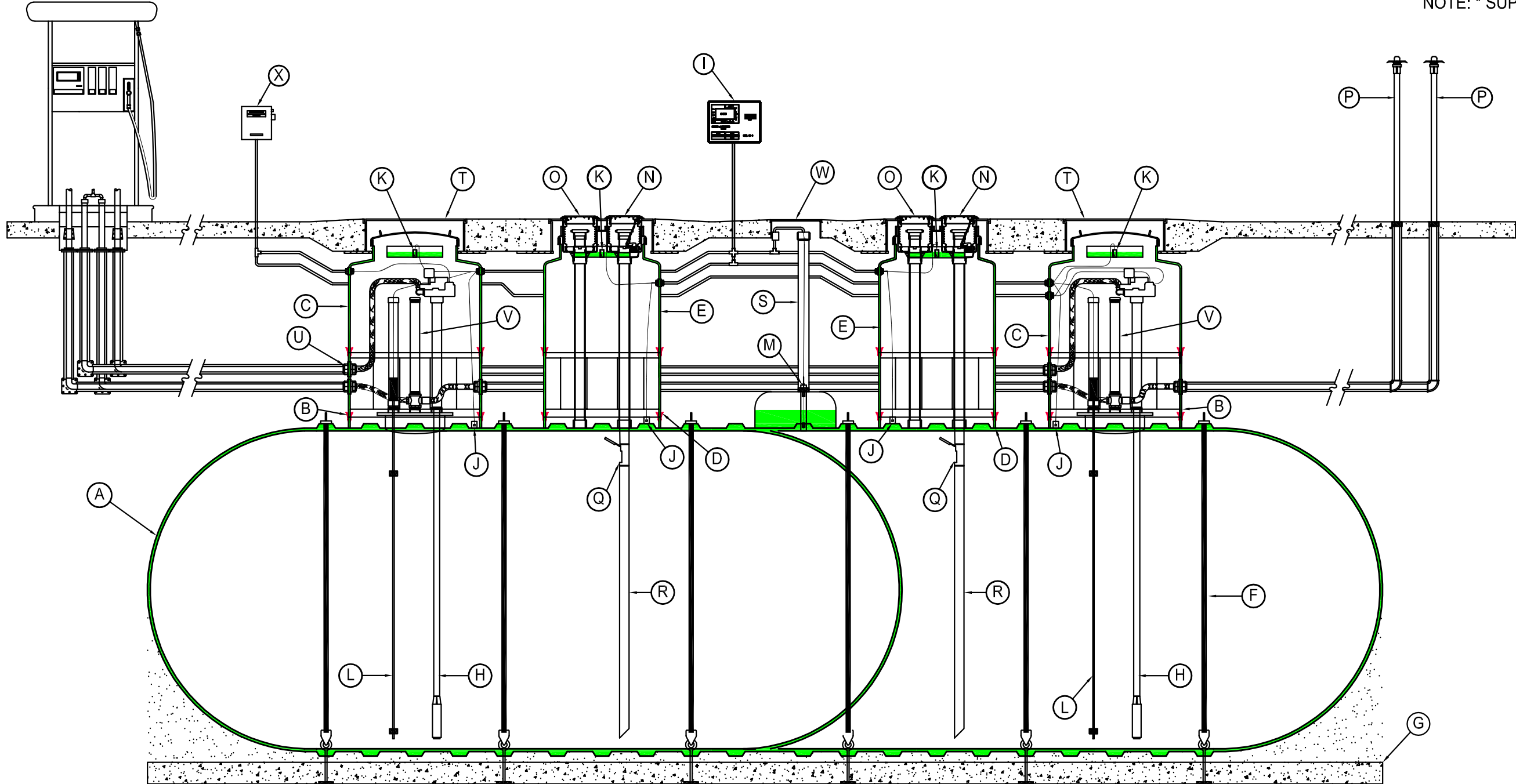
HYDROGUARD® SYSTEM TYPICAL ILLUSTRATION DRAWING MULTI-SUMP SYSTEM (10')-12,000/8,000 GALLON DOUBLE-WALL COMPARTMENT TANK w/ DOUBLE-WALL TURBINE AND FILL/VAPOR SUMPS
