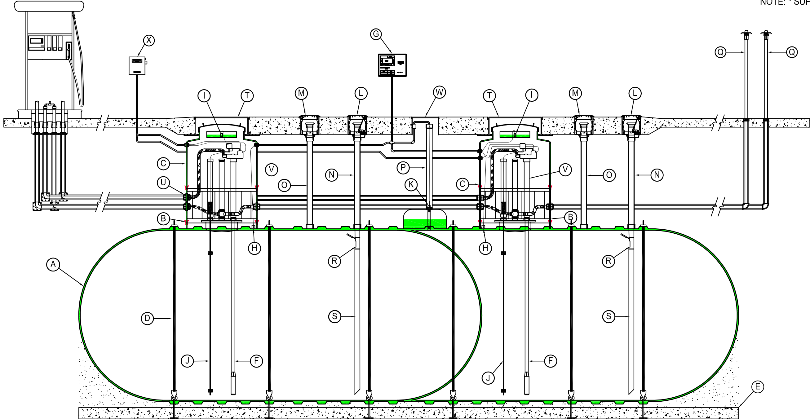
HYDROGUARD® SYSTEM TYPICAL ILLUSTRATION DRAWING SINGLE-SUMP SYSTEM (10')-12000/8000 GALLON DOUBLE-WALL COMPARTMENT TANK w/ DOUBLE-WALL TURBINE SUMPS
