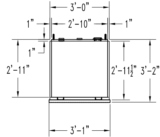
END VIEW
