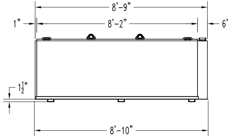
ELEVATION VIEW
