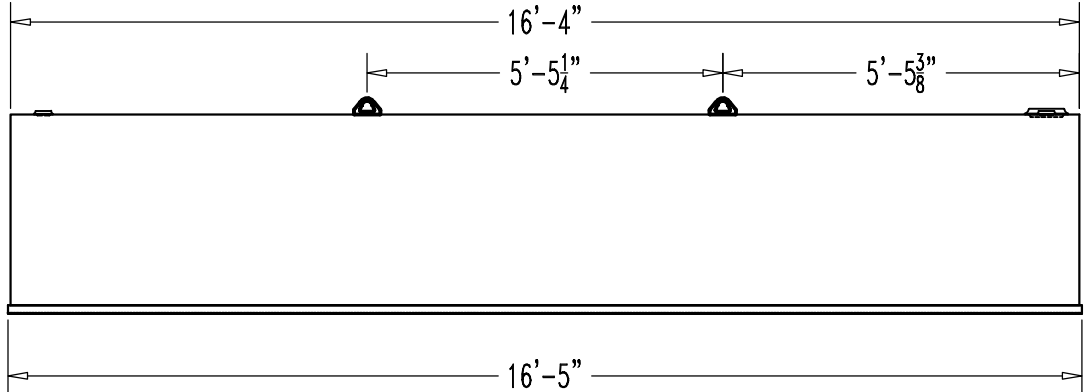
ELEVATION VIEW
