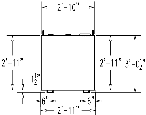
END VIEW
